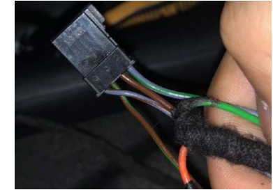
8. Or connect our green line to the original car's blue and green side line, and our orange line to the original car's brown and green side
