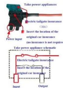
11. Fuse definition diagram
